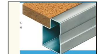
Standard Duty Stepped Beam (2LST) For use with 18mm thick chipboard. Lengths range from 1050mm to 3000mm
